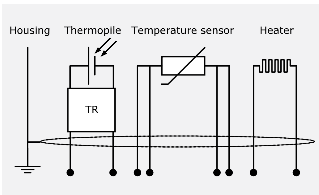
Figure 7.3.1 Electrical diagram of the internal wiring of IR02-TR. The shield is connected to the sensor body.
