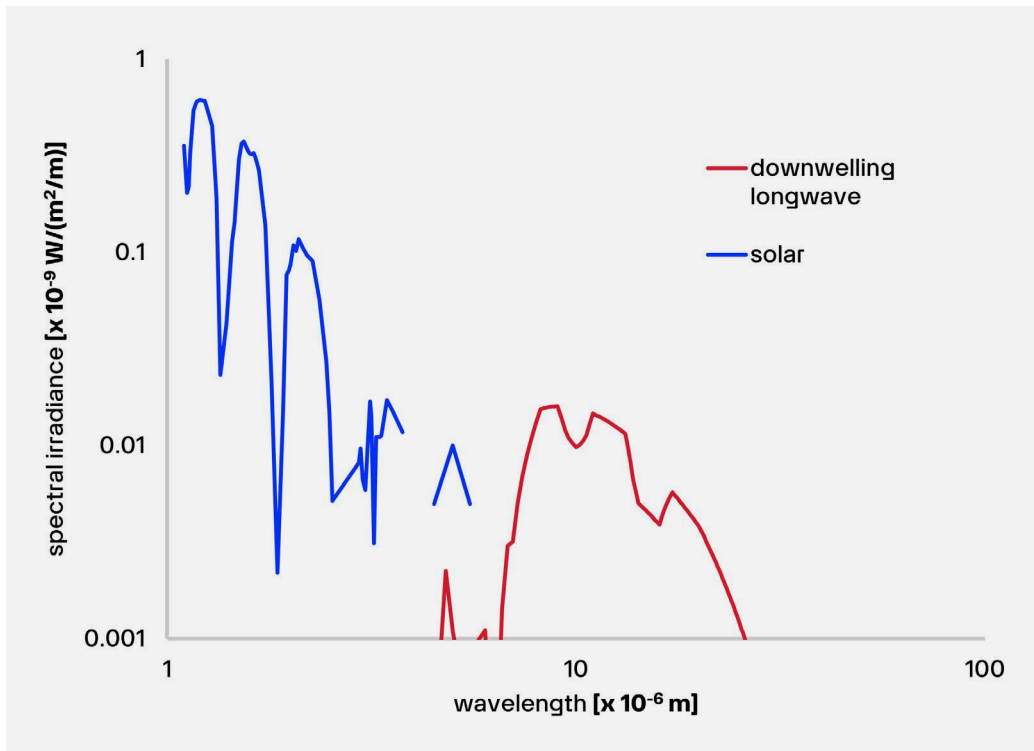
Figure 2.21 Atmospheric radiation as a function of wavelength plotted along two logarithmic axes to highlight the longwave radiation. Longwave radiation is mainly present in the 4 to 50 x 10 -6 m range, whereas solar radiation is mainly present in the 0.3 to 3 x 10 -6 m range. In practice, the two are measured separately using pyrgeometers and pyranometers.
