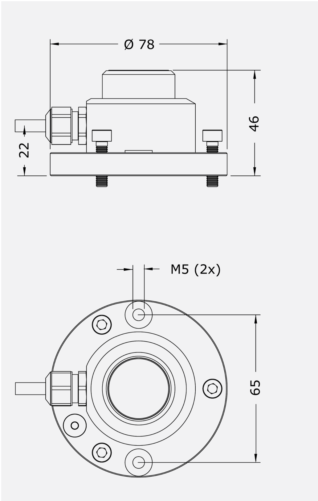
Figure 3.2.1 Dimensions of IR02 in 10^{-3} m.
