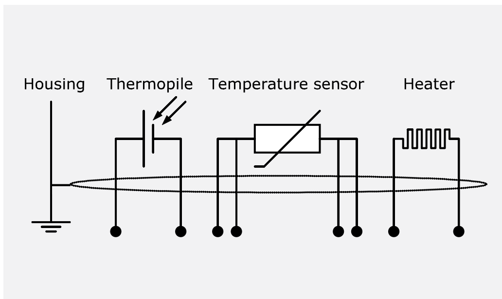
Figure 4.2.1 Electrical diagram of the internal wiring of IR02. The shield is connected to the sensor body.
